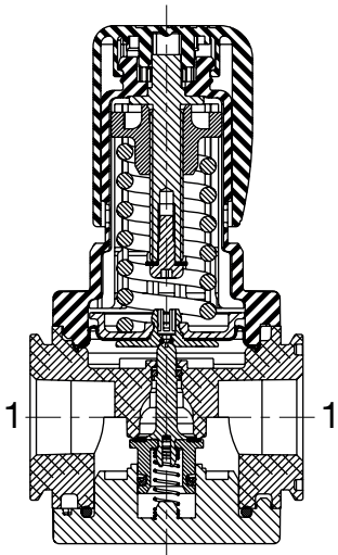
Cross Section - Series 651/652 Manifold Regulator
