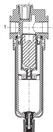
Cross Section - Series 651/652/653 Particulate Filter
