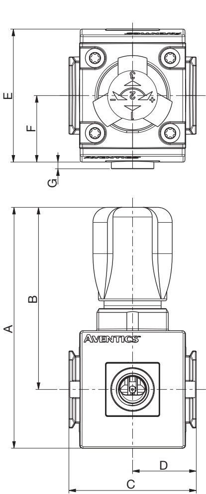
Dimensions: mm (inches) Series 651/652 Manifold Regulator
