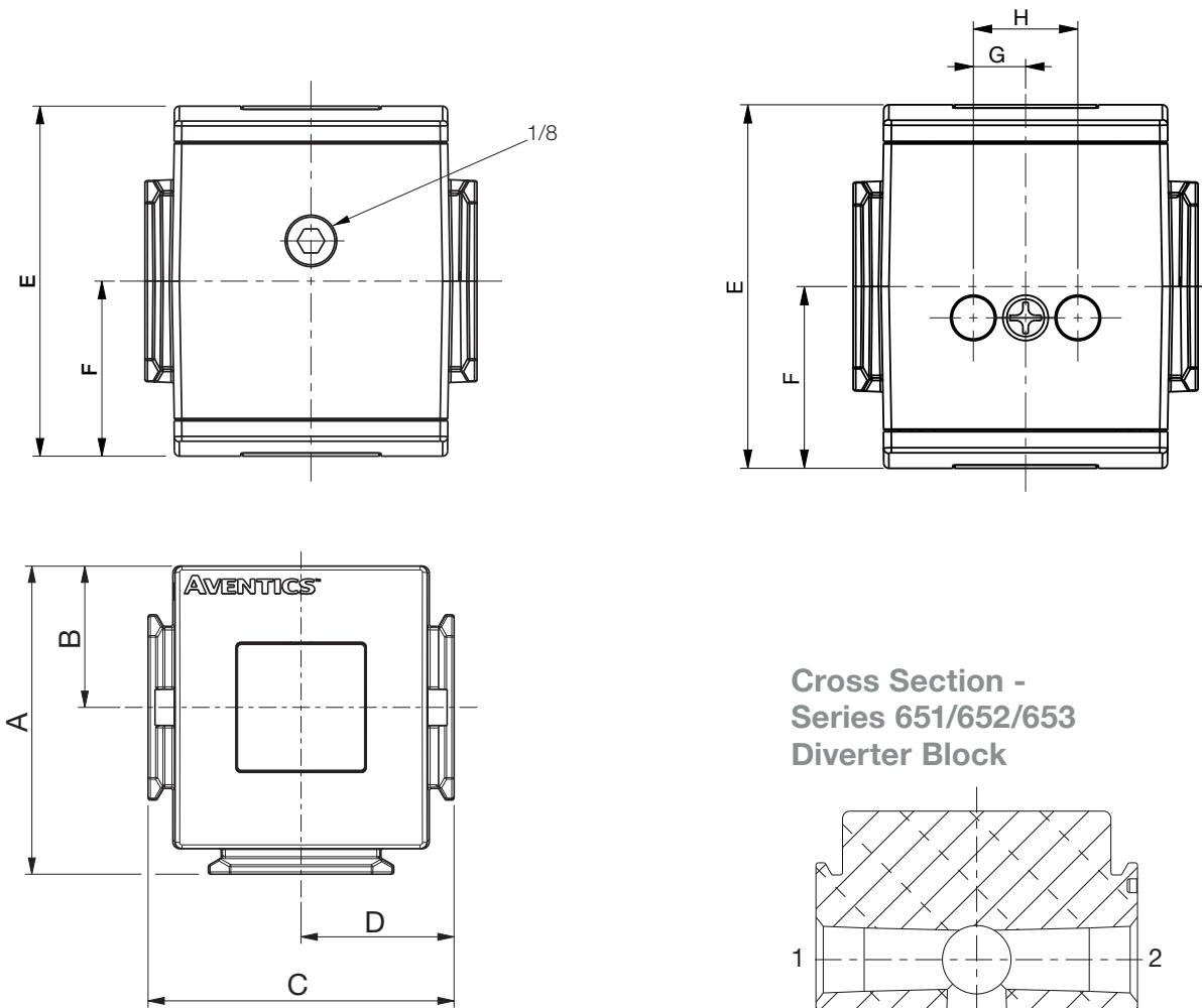
Dimensions: mm (inches) Series 651/652/653 Diverter Block
