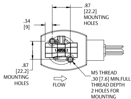
Const. Ref. 3, 4 (1/4" Pipe)
