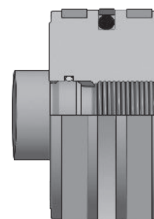
Miller KP Filled PTFE Piston Seal
