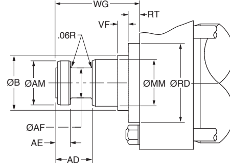
Thread Style 55 1
