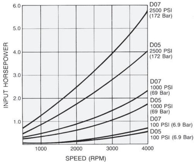
D05/D07 Horsepower/Speed
