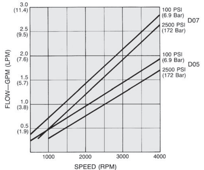
D05/D07 Flow/Speed
