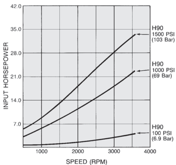
H90 Horsepower/Speed
