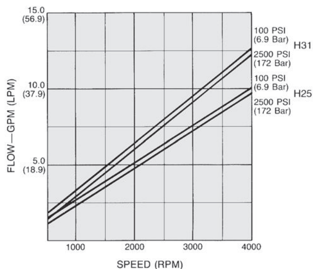
H25/H31 Flow/Speed
