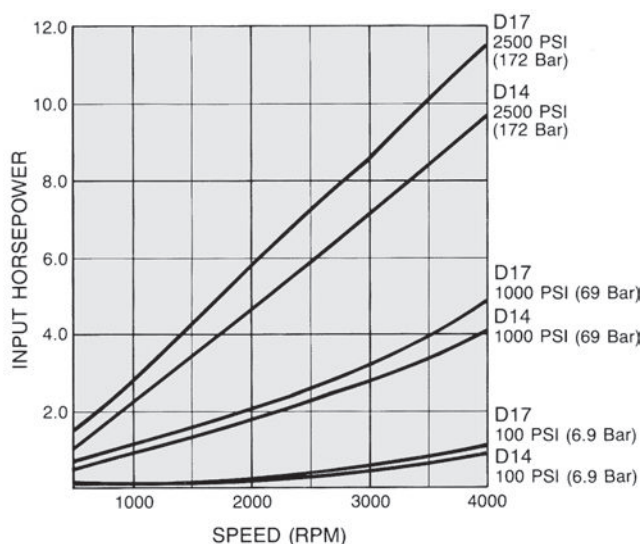
D14/D17 Horsepower/Speed
