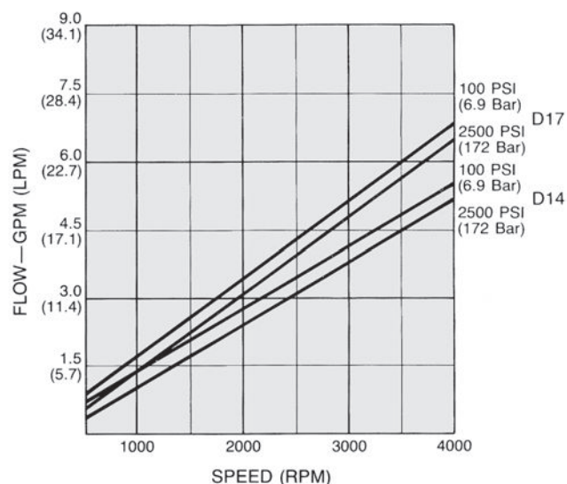
D14/D17 Flow/Speed
