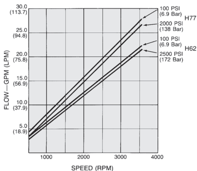
H62/H77 Flow/Speed
