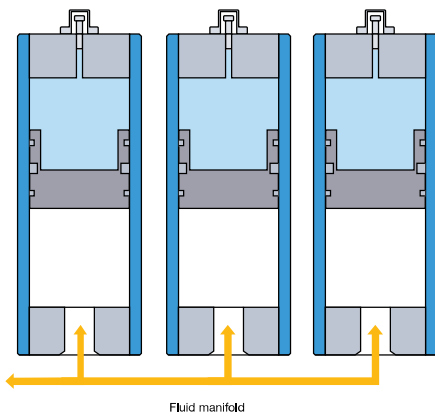
Fig. 9 Multiple accumulators manifolded together offer high system flow rates
