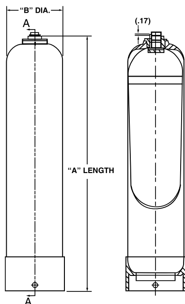
Polyglass KleenVent
