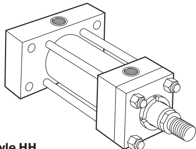
Style HH Cap Rectangular Flange (ISO Style ME6)
