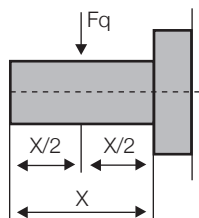
Radial Load Diagram
