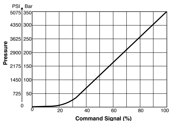
Pressure vs. Input Current
